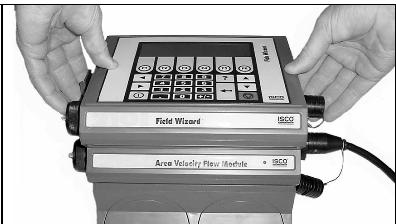
Figure 2-12: Push down and lock the latch
