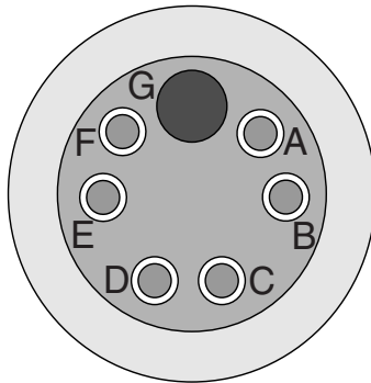
Figure 1-4 Model 2101 Field Wizard Connector Pins
