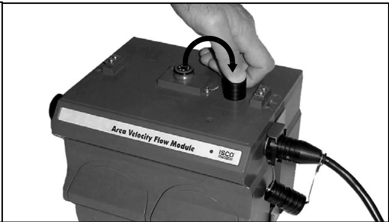
Figure 2-10: 2100 Series Module - uncap the connector
