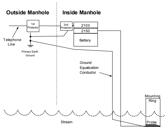
Figure 2: Preferred Installation Configuration
