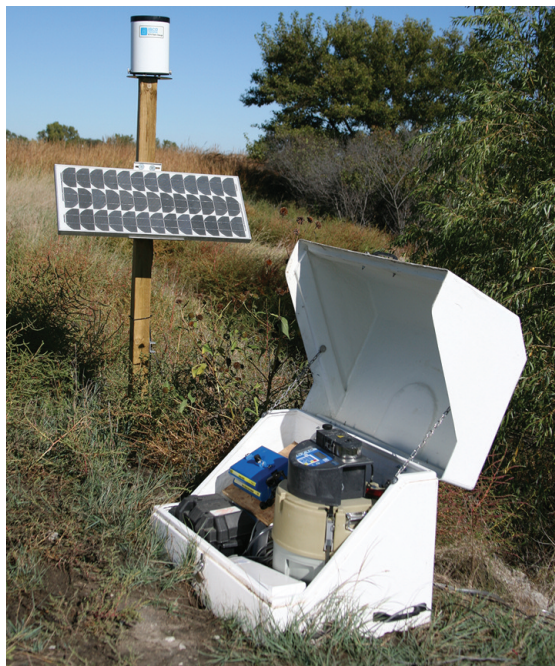
The 2105 system shown above interfaces a rain gauge, flow meters, automatic sampling, and a multi-parameter sonde.
