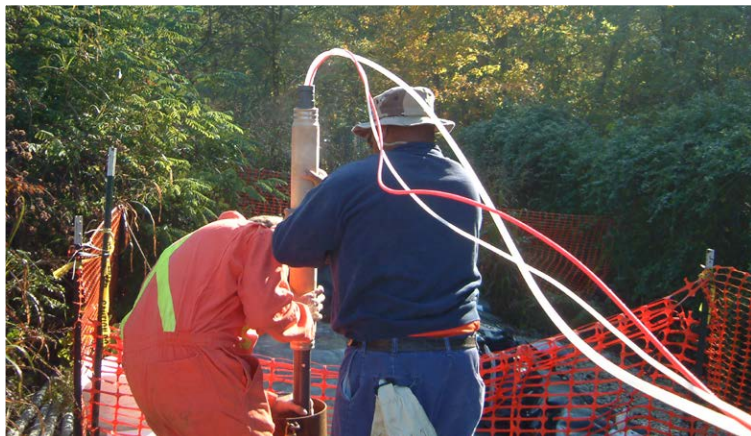
Figure 4-4 Initial Section Being Installed Down-hole
