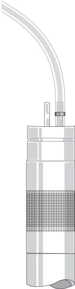
Figure 6-3 5/8"OD x 1/2"ID tubing attached over 3" of 1/2"OD x 3/8"ID tubing to Port Stem Using Oetiker #17 Clamp
