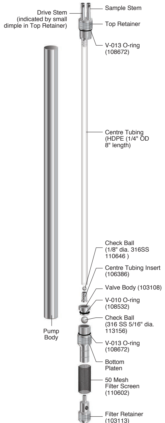
5/8" Double Valve Pump Mk3 (#103104)
