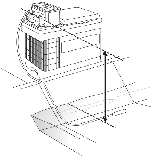
Figure 1-3 Measuring Suction Head Height
