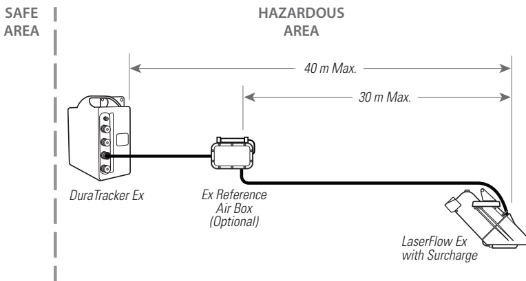
Figure 2-9 360 LaserFlow Ex Sensor with Surcharge Sensor
