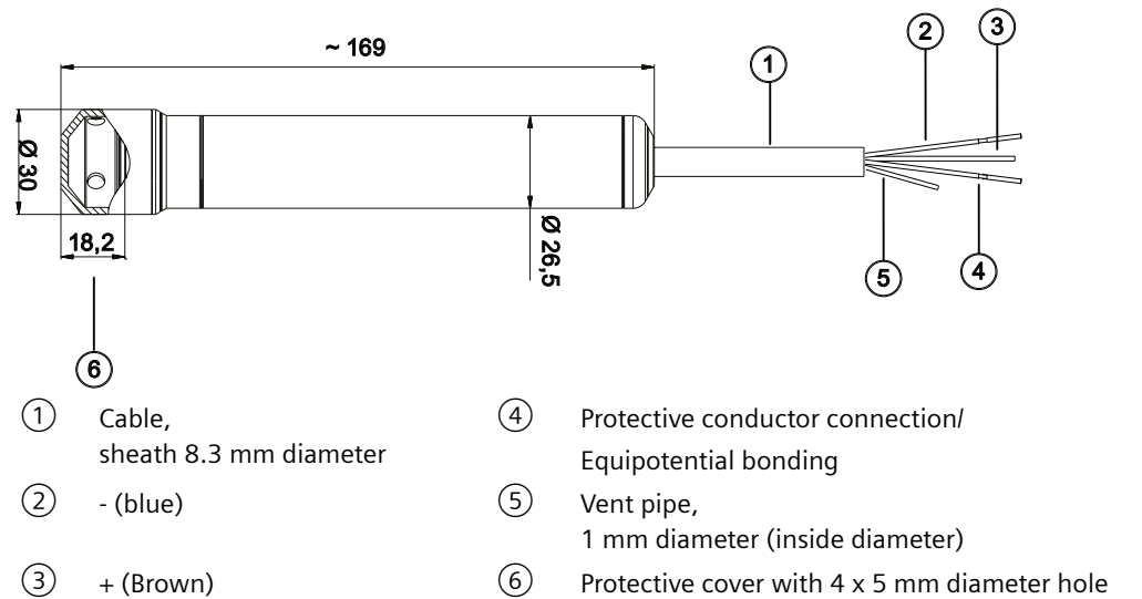
Figure 9-2 Pressure transmitter with protective cover made of stainless steel, dimensions in mm
