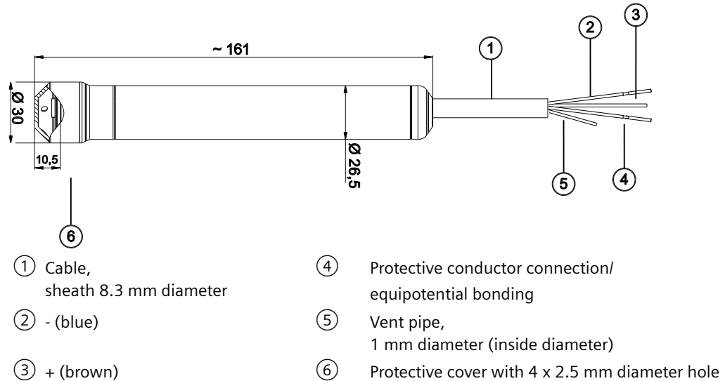
Figure 9-1 Pressure transmitter with protective cover made of PPE/ETFE, dimensions in mm
