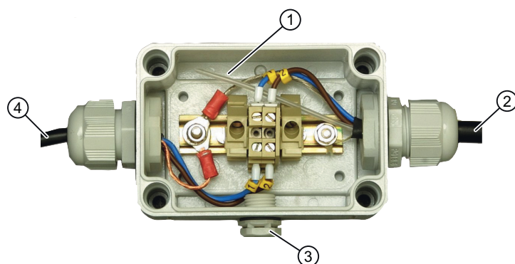
Figure 5-1 Cable box (example for applications in hazardous area)
